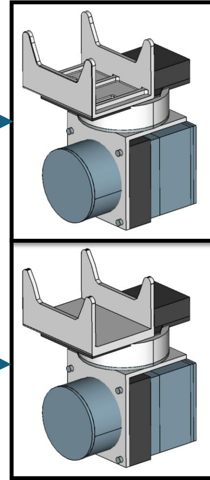
PPS6 Prism off Faces: 268
